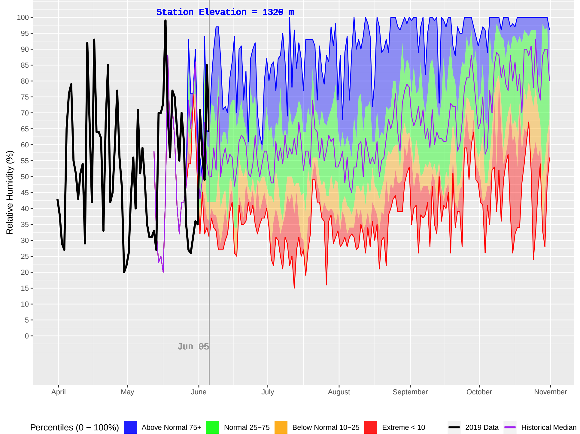
PINE CREEK (938) : Historical (2006–2018) and Current (2019) Daily Relative Humidity
