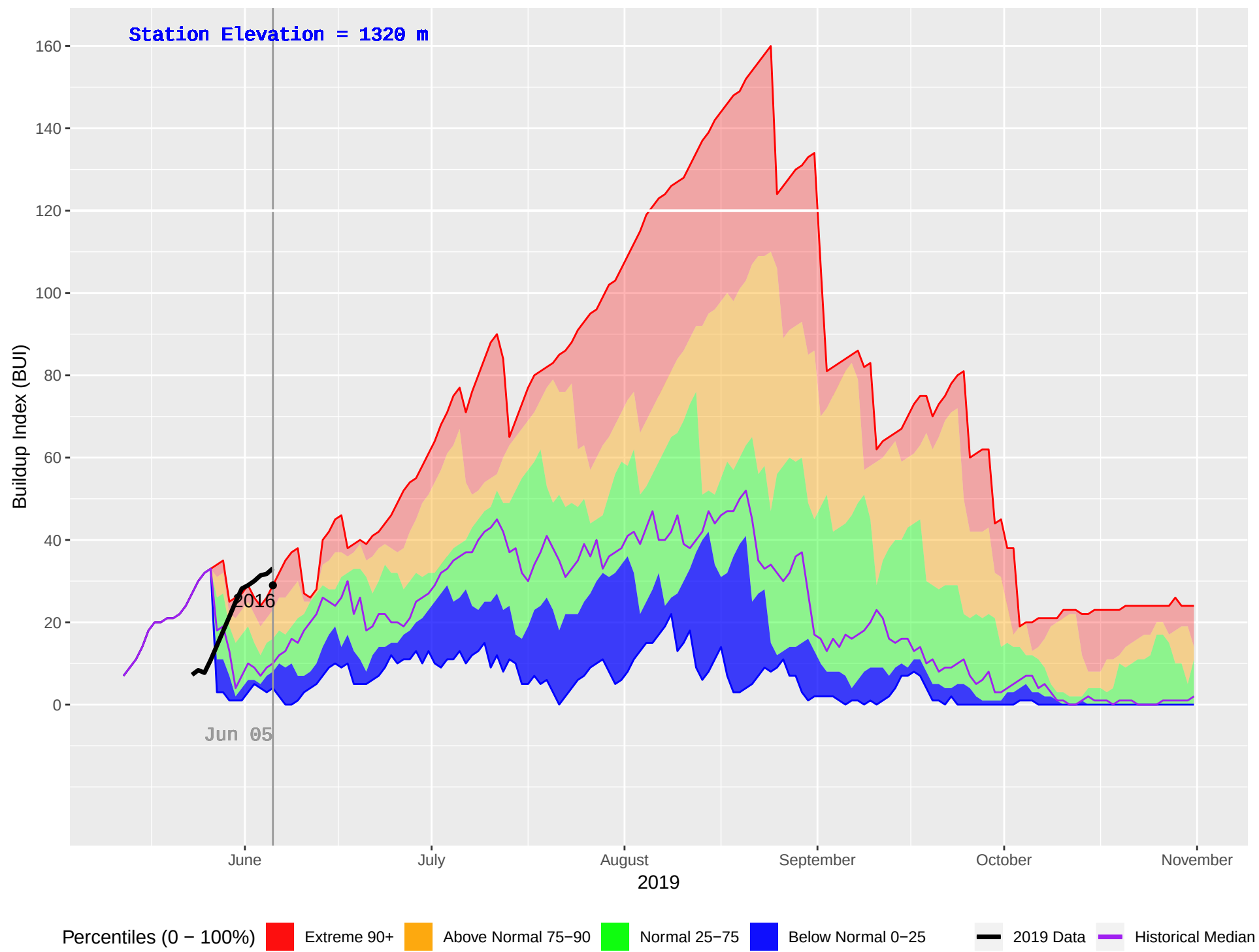
PINE CREEK (938) : Historical (2006–2018), Current (2019) Daily Buildup Index (BUI)
