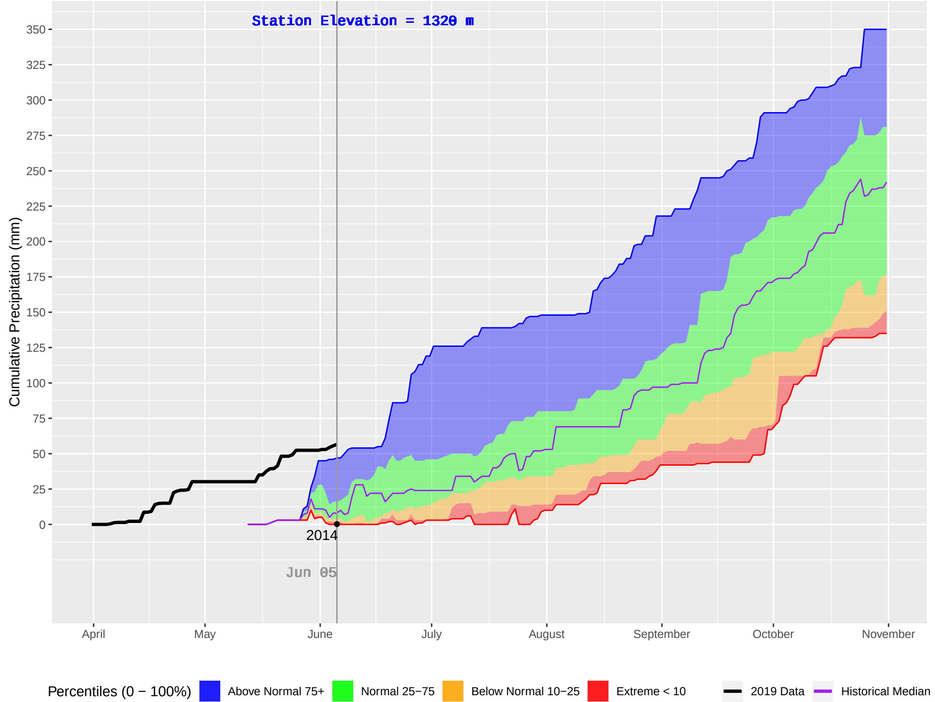
PINE CREEK (938) : Historical (2006–2018), Current (2019) Daily Cumulative Precipitation
