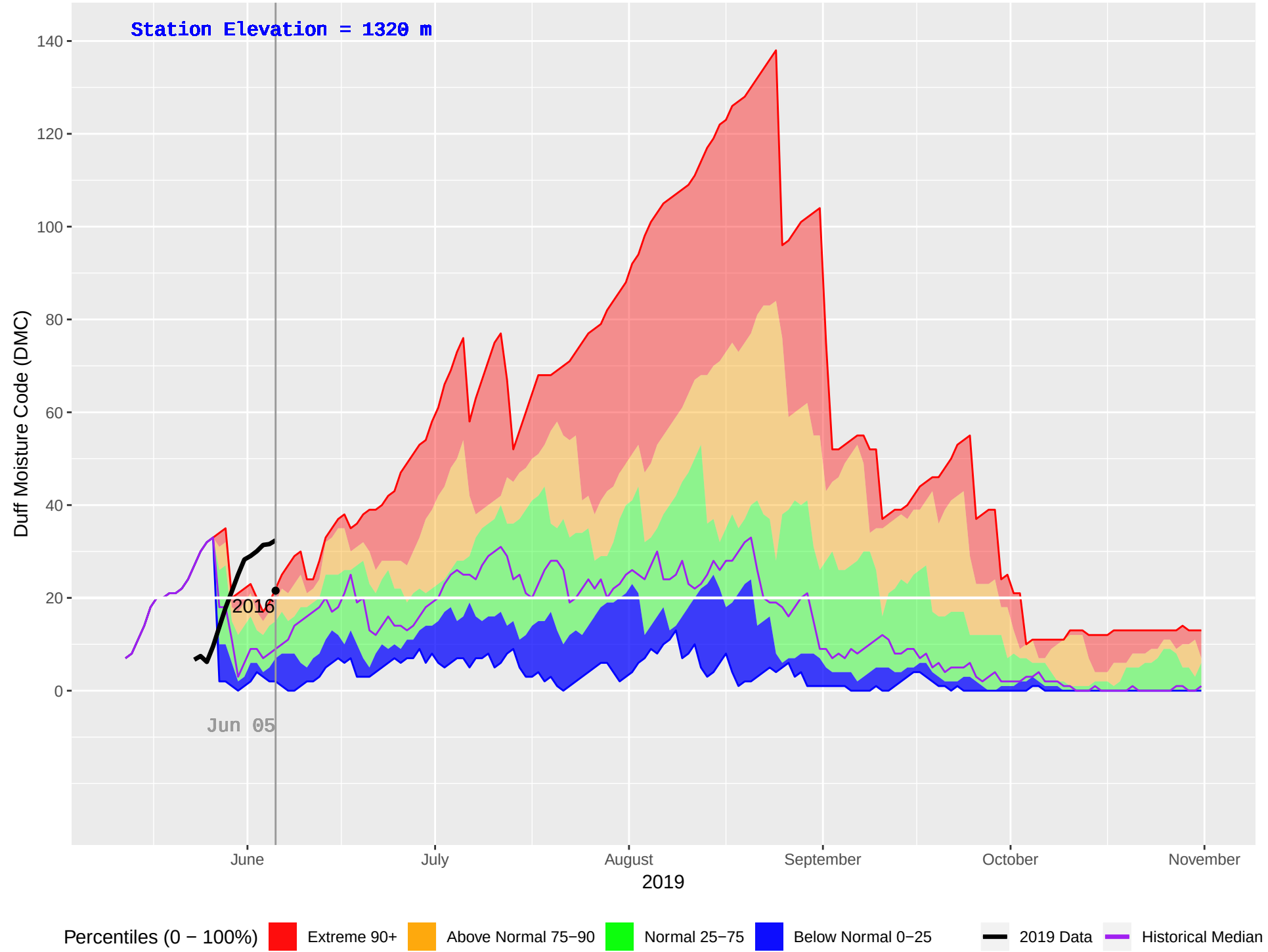
PINE CREEK (938) : Historical (2006–2018), Current (2019) Daily Duff Moisture Code (DMC)
