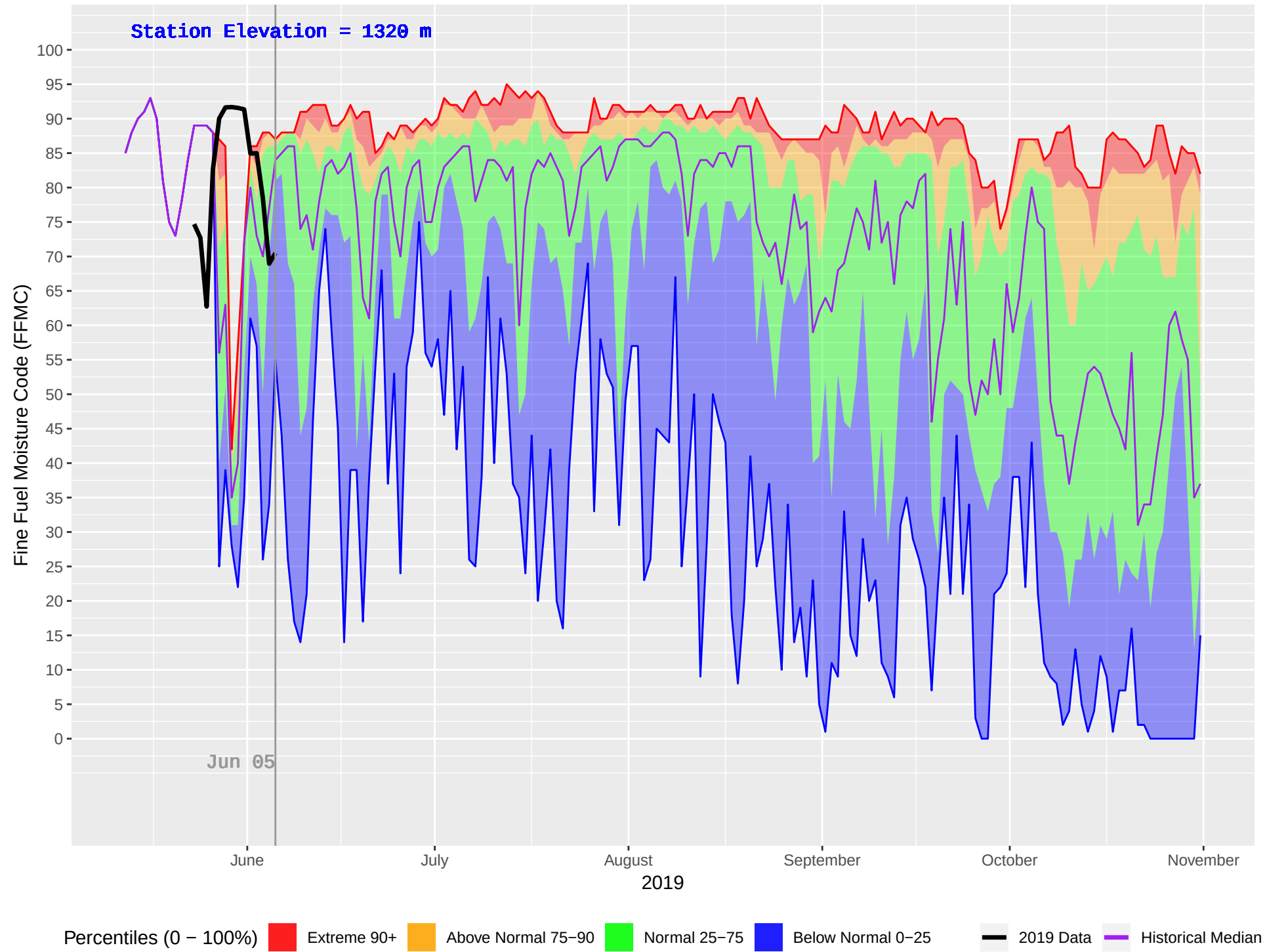
PINE CREEK (938) : Historical (2006–2018) and Current (2019) Daily Fine Fuel Moisture Code (FFMC)
