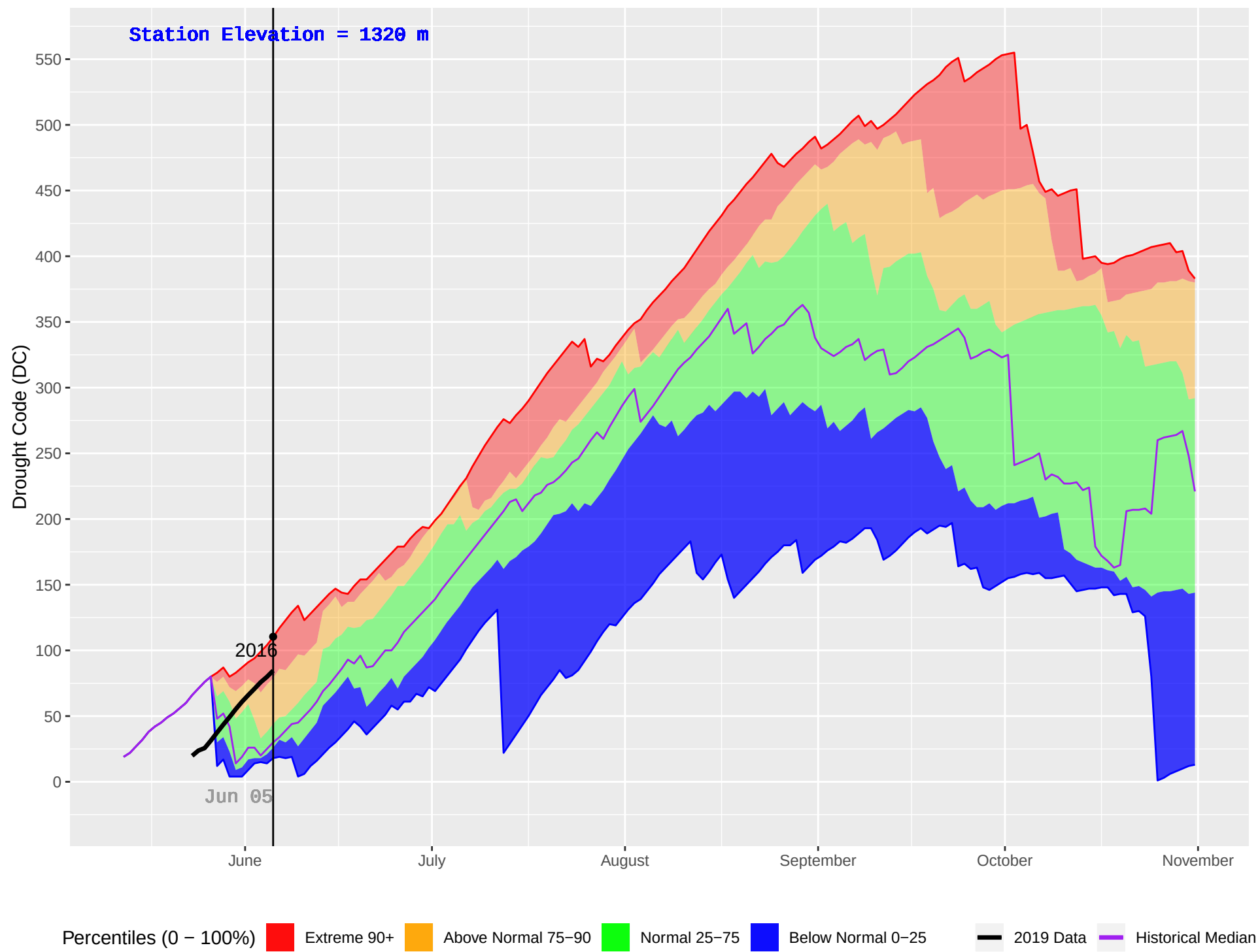
PINE CREEK (938) : Historical (2006–2018) and Current (2019) Daily Drought Code (DC)
